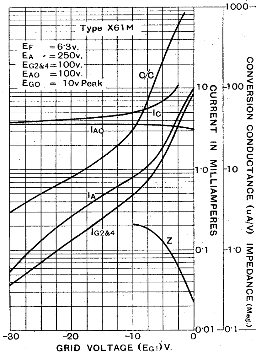
CHARACTERISTIC CURVES OF AVERAGE VALVE.
